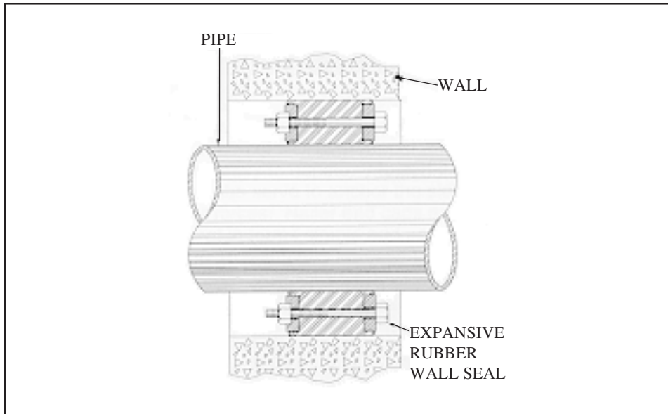
Figure 3.4.3F: Examples of an expansive rubber wall or floor penetration seal Source: PROJEX GROUP Pty. Ltd., Unit 3/39 Rhodes Street, Hillsdale NSW, Australia 2036
