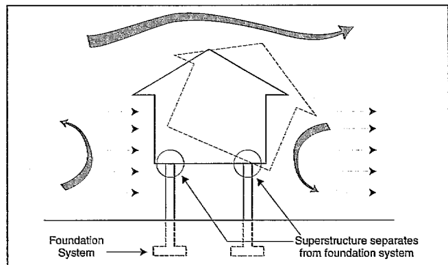
Horizontal wind forces and associated suction (negative forces) on the rear wall can cause an overturning effect.
