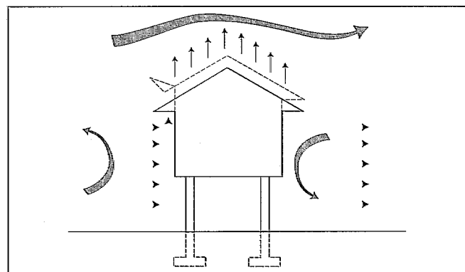
As the wind blows over the roof, its increasing speed can draw the roof upward and off the house. Wind forces also stress connections between structural members, such as between piles and floor beams, weakening the structure.
