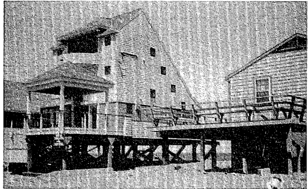
Residences are typically elevated on pressure-treated, cross-braced wood piles. One local contractor constructs over 25 residential elevation projects a year.
