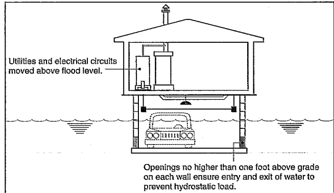
In a typical residential elevation, an eight-foot or higher area below the house can be used for parking, access, and limited storage during non-flood conditions.
