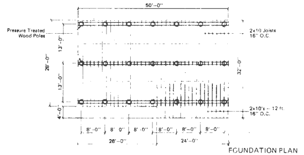
FOUNDATION PLAN
