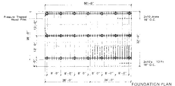
FOUNDATION PLAN
