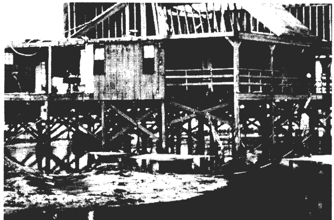
Figure 4.23. Diagonal Bracing
